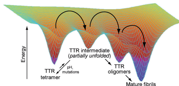
Figure 1. A free-energy landscape depicting the prominent conformational states of TTR. Arrows between energy wells denote conformational excursions of TTR from one state to another.
